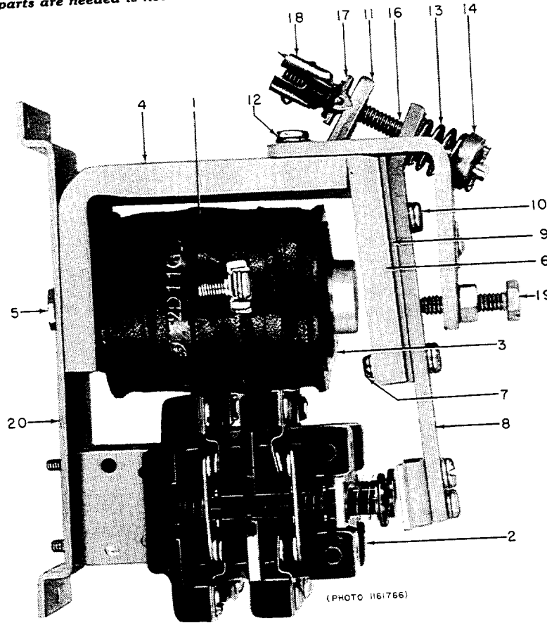
IC2820-A100B Relay
