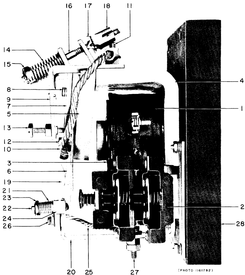
IC2800-A501A contactor
